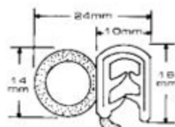
LHCW0015 CAR DOOR SPONGE
