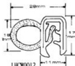
LHCW0012 CAR DOOR SPONGE
