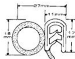
LHCW0017 CAR DOOR SPONGE
