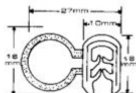
LHCW0018 CAR DOOR SPONGE
