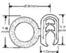
LHCW0016 CAR DOOR SPONGE
