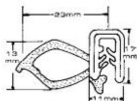
LHCW0011 CAR DOOR SPONGE
