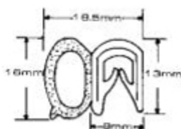
LHCW0019 CAR DOOR SPONGE
