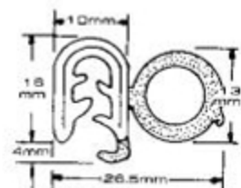
LHCW0014 CAR DOOR SPONGE
